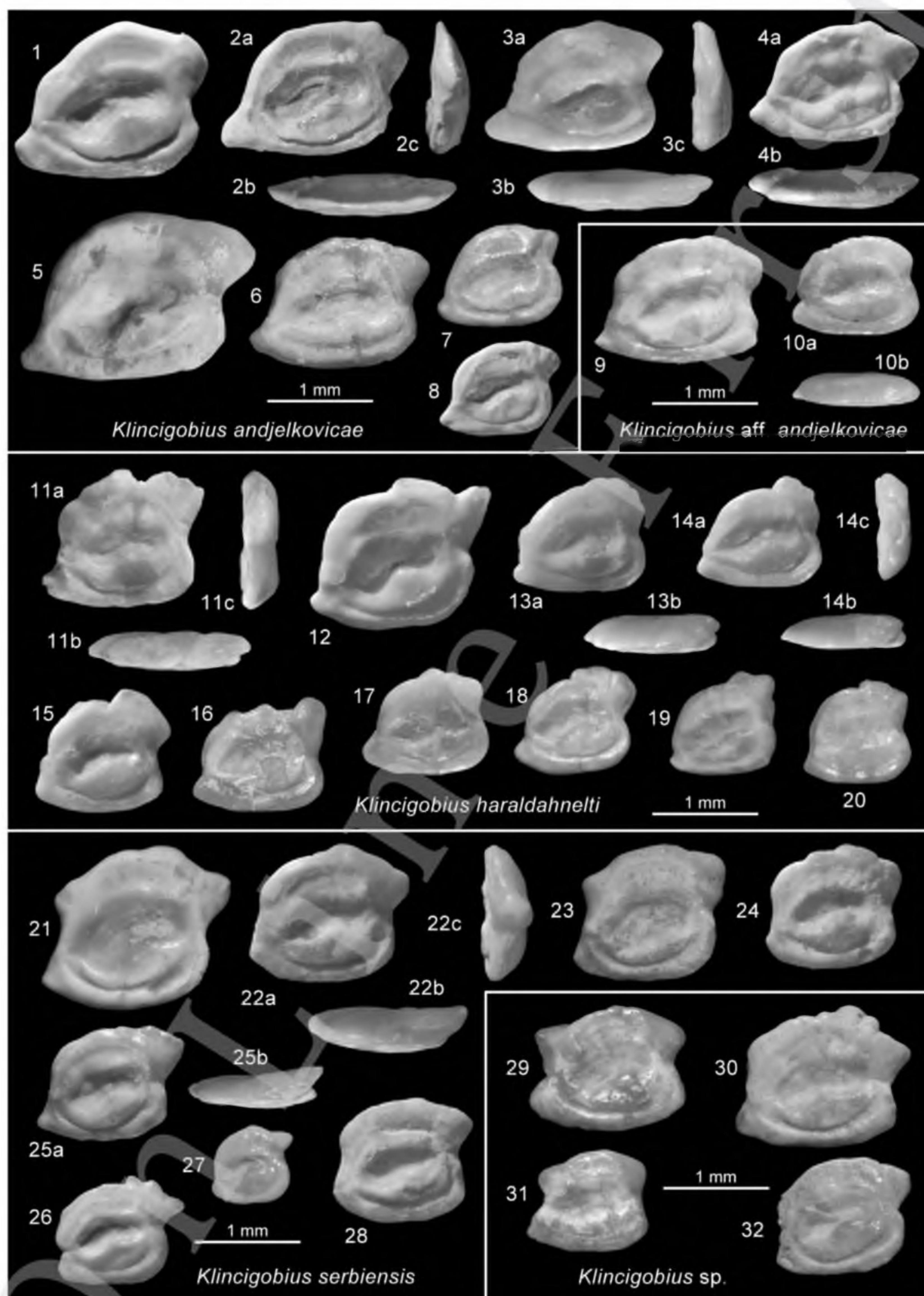
Fig. 5. Otoliths of Klincigobius from Vračević; 1–8. Klincigobius andjelkovicae BRADIĆ-MILINOVIĆ, AHNELT & SCHWARZHANS 2019, NHMB-NP 239; 9–10. Klincigobius aff. andjelkovicae BRADIĆ-MILINOVIĆ, AHNELT & SCHWARZHANS 2019, NHMB-NP 333; 11–20. Klincigobius haraldahneli n. sp., holotype (14), NHMB-NP 342; paratypes (11–13, 15–20), NHMB-NP 334; 21–28. Klincigobius serbiensis (GAUDANT, 1998), NHMB-NP 335; 29–32) Klincigobius sp., NHMB-NP 336.
