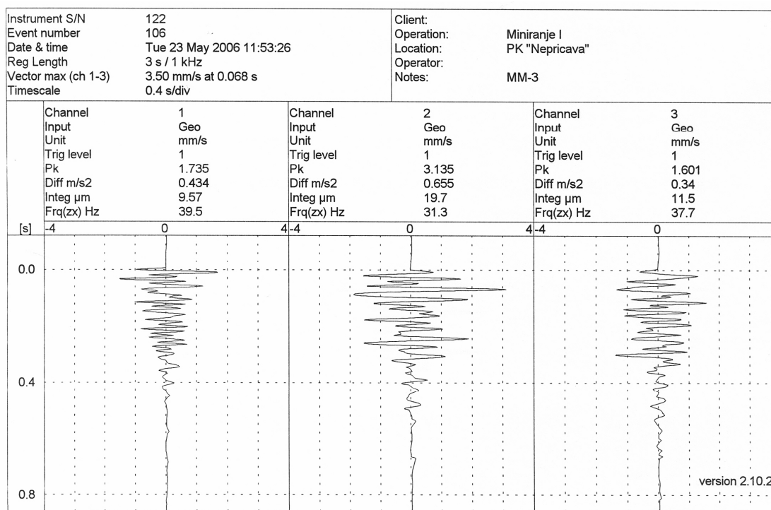
Figure 1. Recording of oscillation velocity of the ground intended for blasting No. I—measuring point No. 3 at PK Nepričava.
