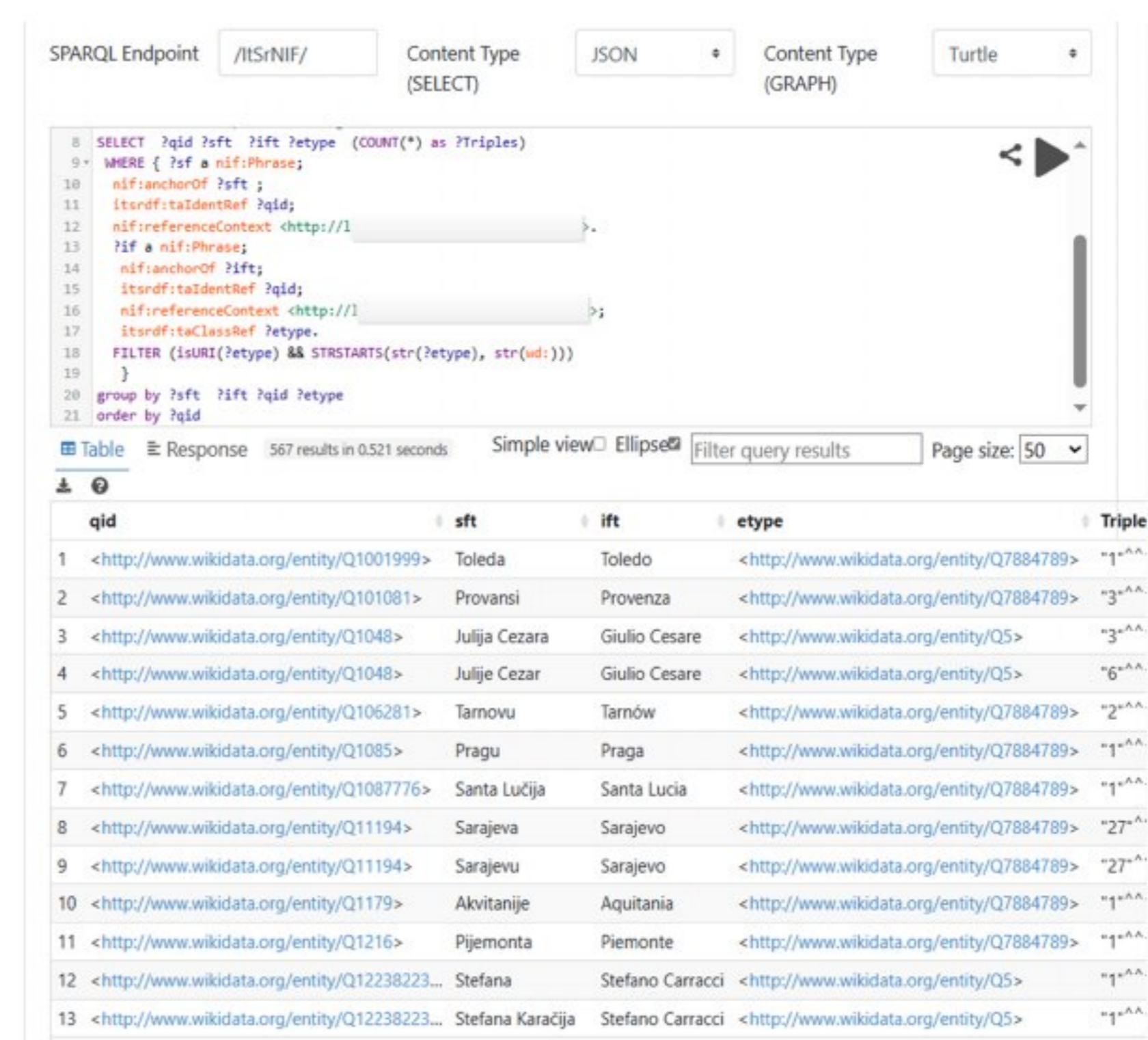
Figure 4: SPARQL query with aligned sentences
