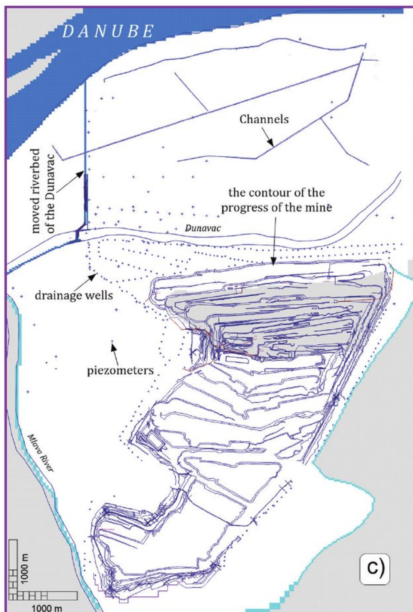
Fig. 1. Presentation of the model domain, the types of boundary conditions, the progress of surface mining, and the state of the drainage system for selected time sections: a, 1998; b, 2008; c, 2018; d, 2022
